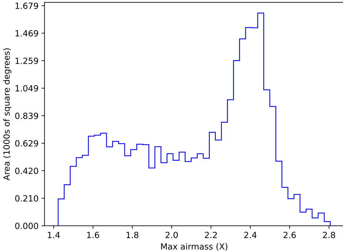
noroll_v3.4_10yrs All sky r band: Max airmass
