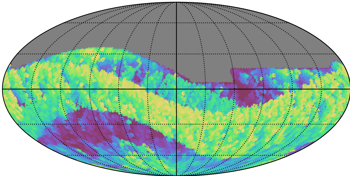
noroll_v3.4_10yrs All sky i band: Max airmass
