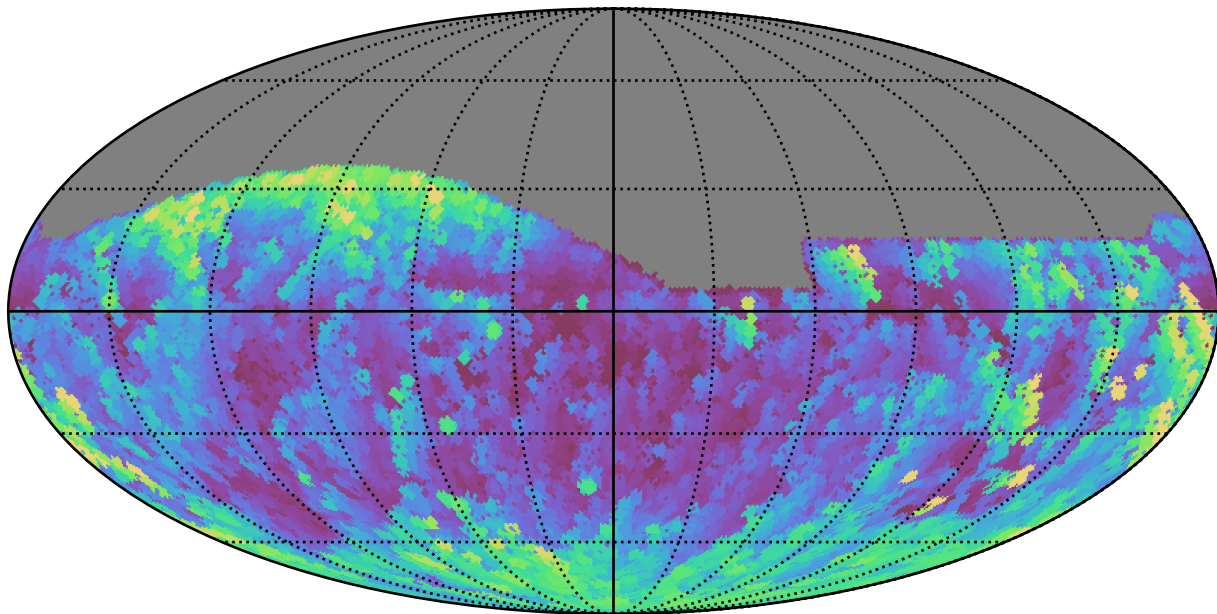
noroll_v3.4_10yrs All sky g band: Max airmass
