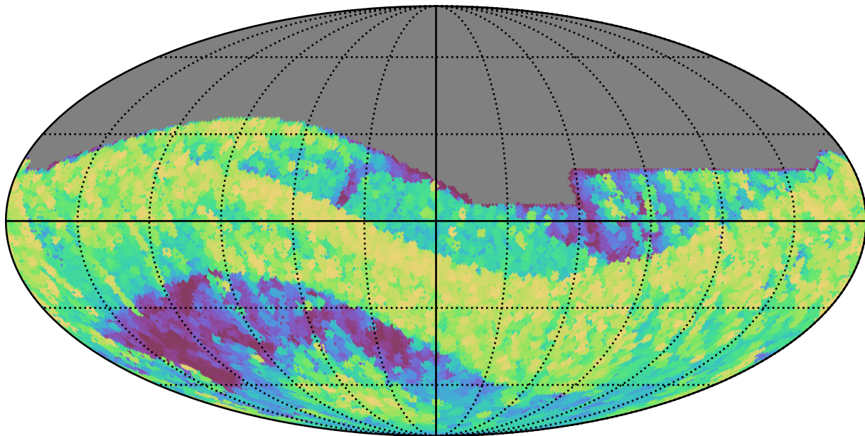
noroll_v3.4_10yrs All sky all bands: Max airmass
