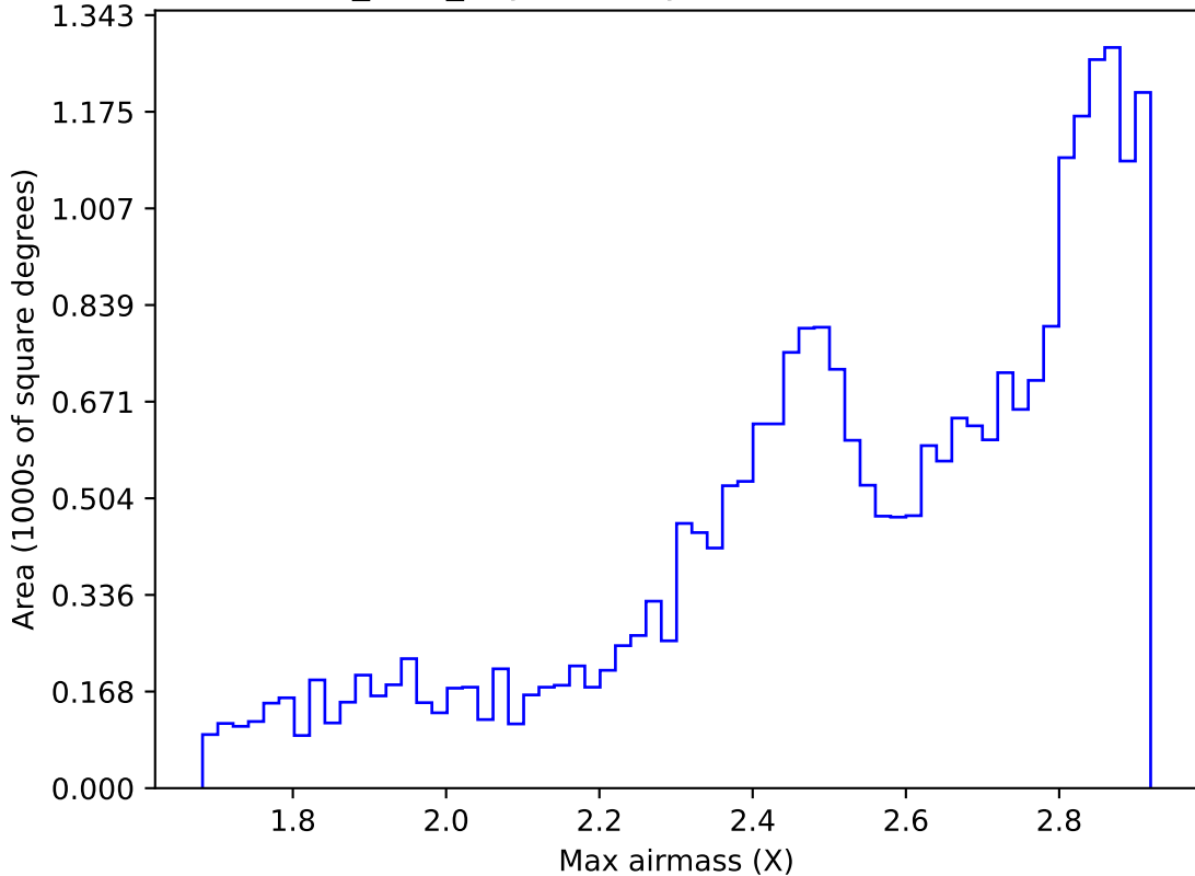
noroll_v3.4_10yrs All sky all bands: Max airmass
