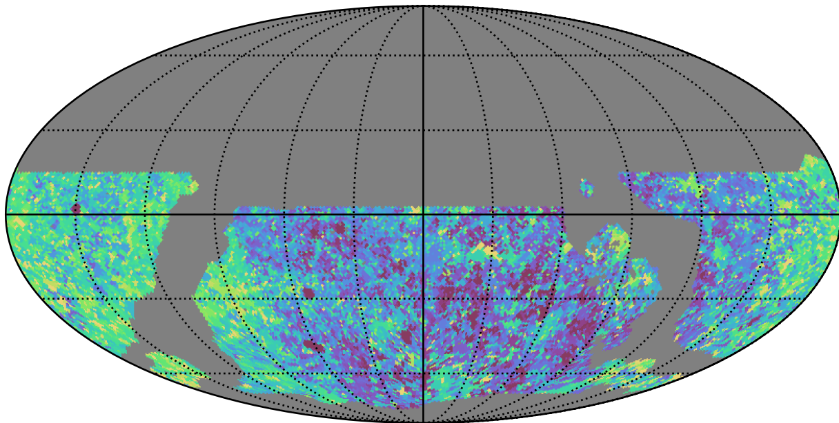
noroll_v3.4_10yrs WFD z band: Max Inter-Night Gap
