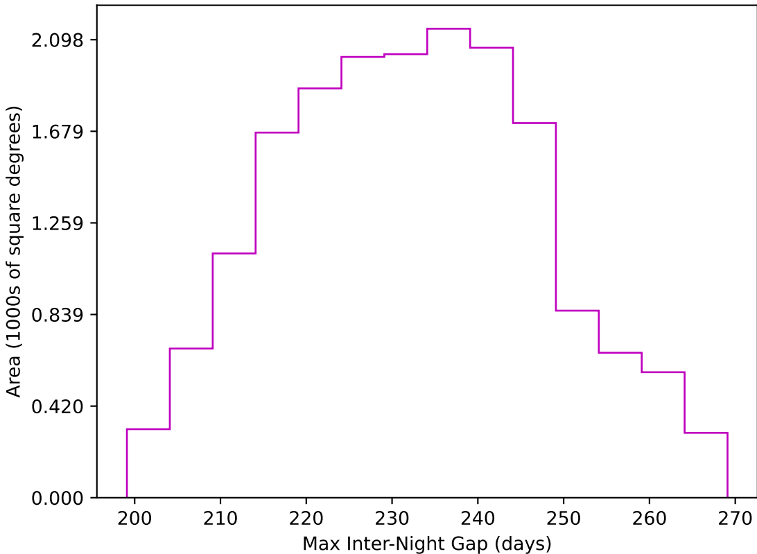
noroll_v3.4_10yrs WFD z band: Max Inter-Night Gap
