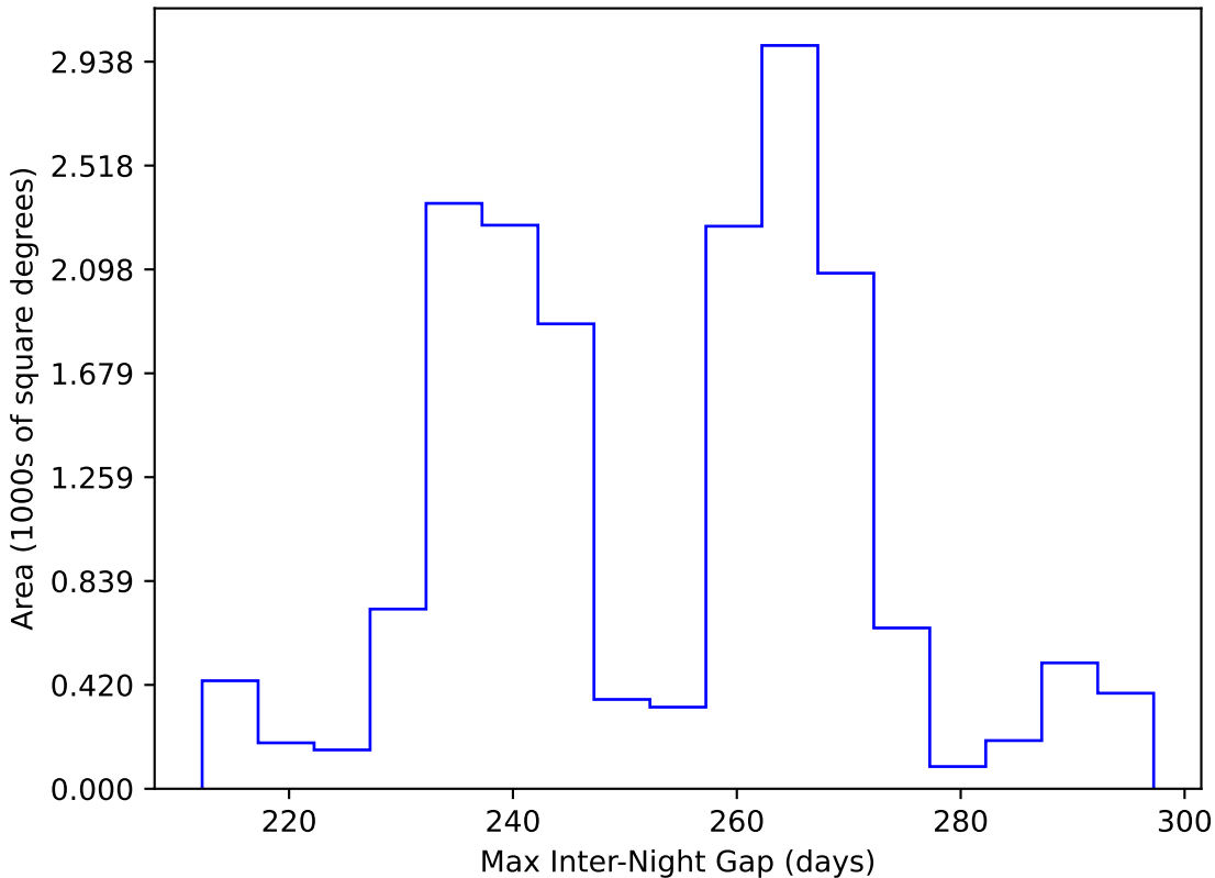
noroll_v3.4_10yrs WFD y band: Max Inter-Night Gap
