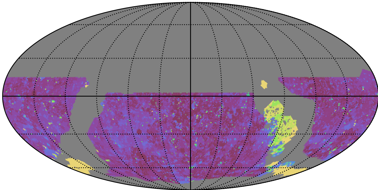
noroll_v3.4_10yrs WFD u band: Max Inter-Night Gap
