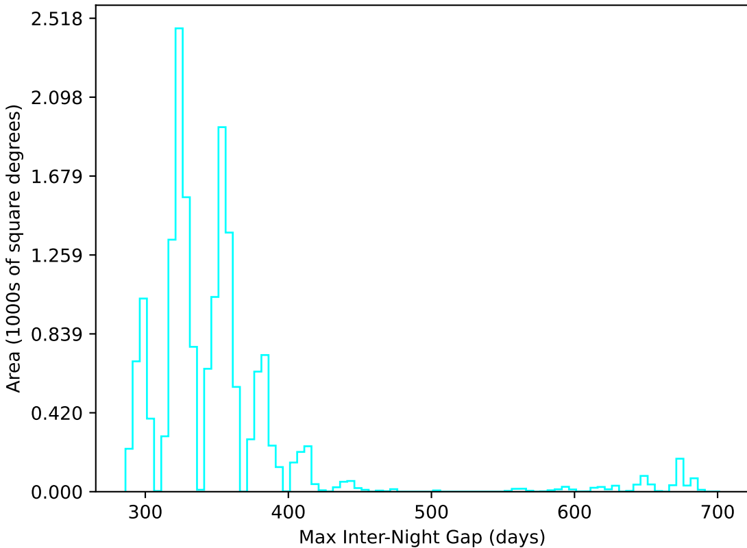
noroll_v3.4_10yrs WFD u band: Max Inter-Night Gap
