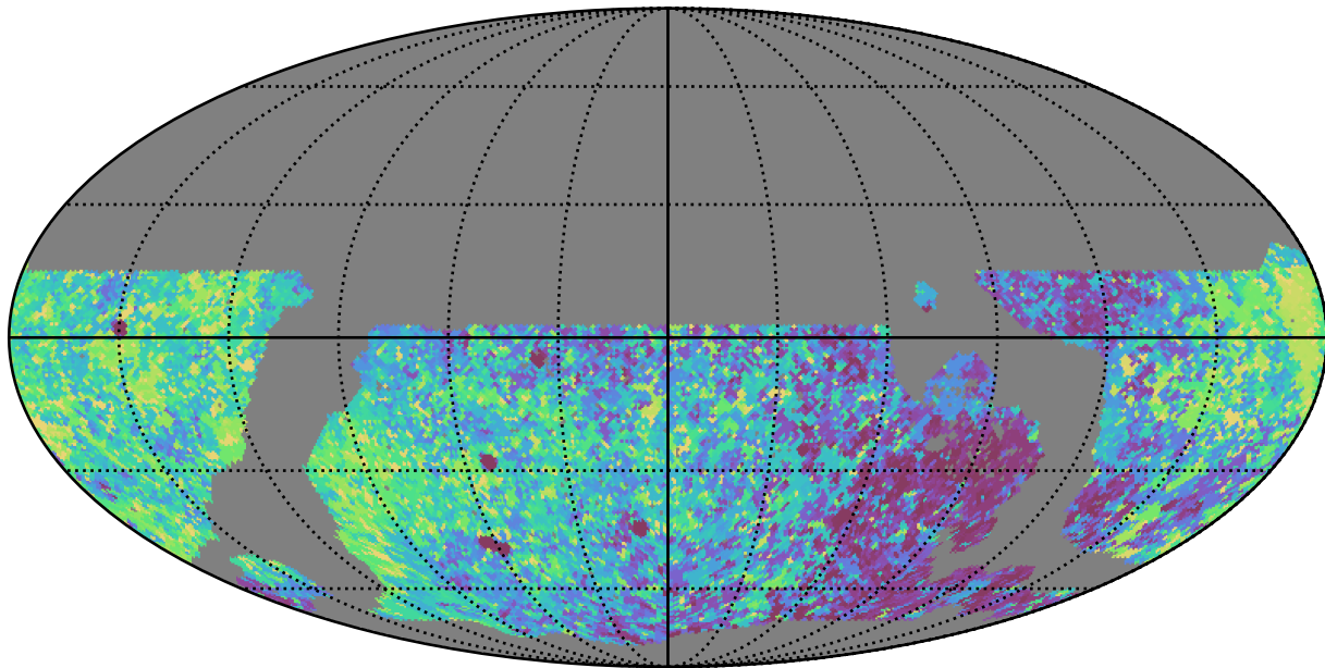
noroll_v3.4_10yrs WFD r band: Max Inter-Night Gap
