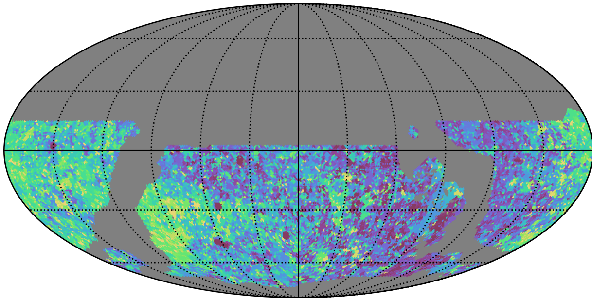
noroll_v3.4_10yrs WFD i band: Max Inter-Night Gap
