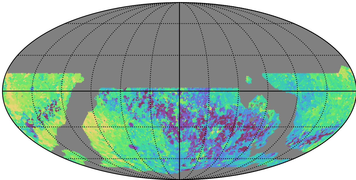
noroll_v3.4_10yrs WFD all bands: Max Inter-Night Gap
