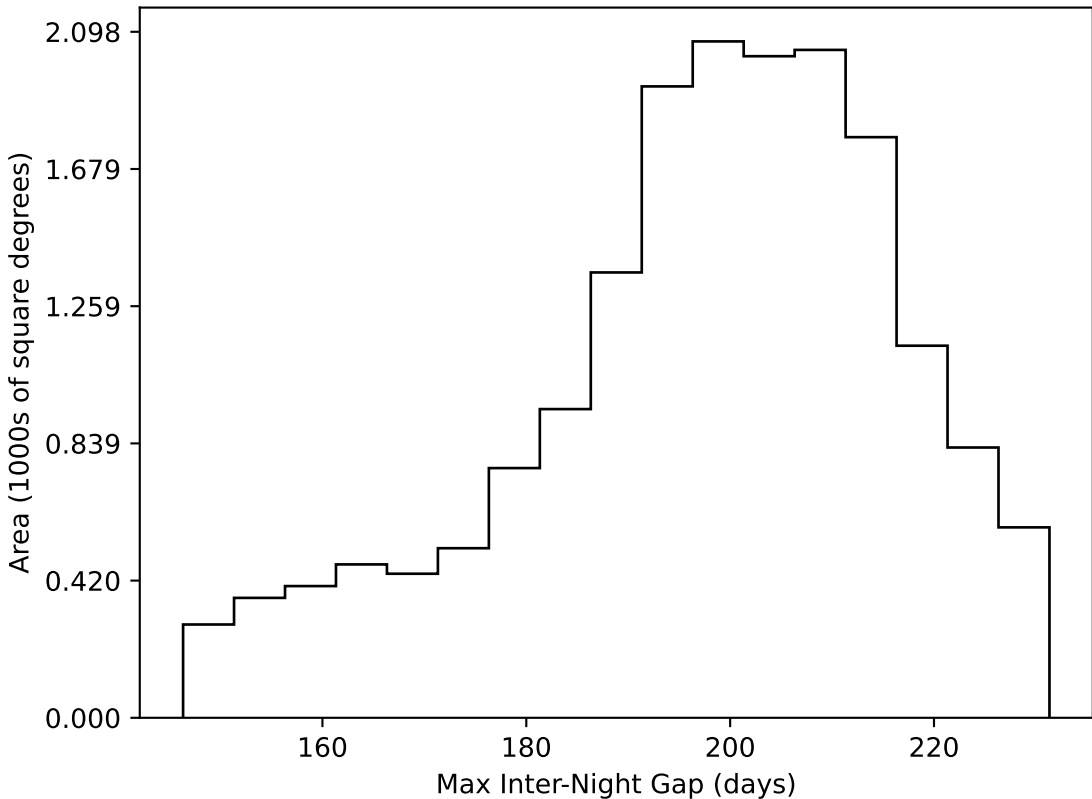
noroll_v3.4_10yrs WFD all bands: Max Inter-Night Gap
