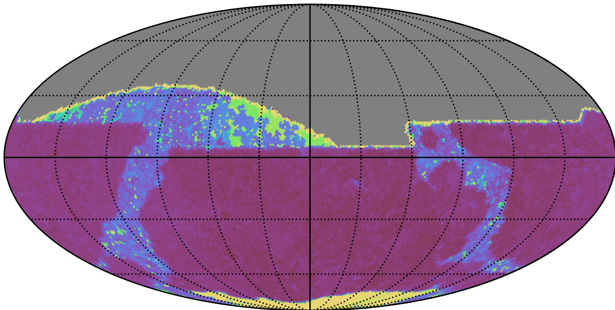
noroll_v3.4_10yrs All sky z band: Max Inter-Night Gap
