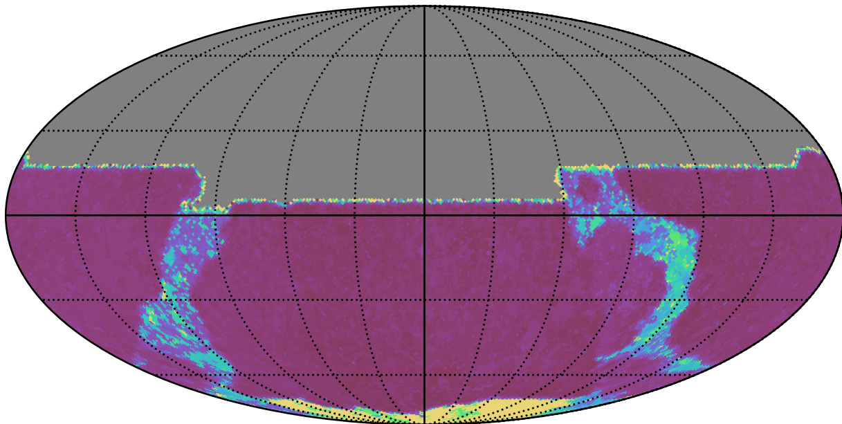
noroll_v3.4_10yrs All sky y band: Max Inter-Night Gap
