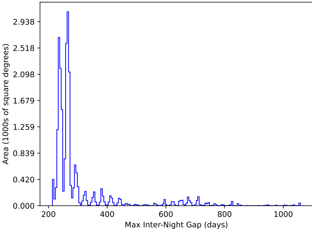
noroll_v3.4_10yrs All sky y band: Max Inter-Night Gap
