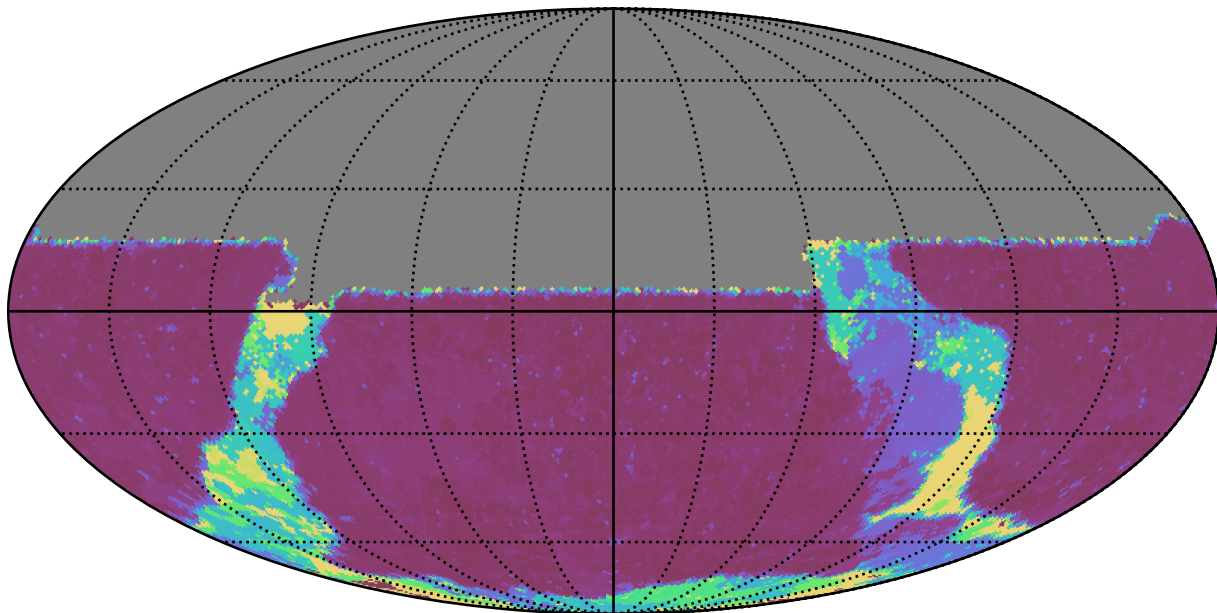
noroll_v3.4_10yrs All sky u band: Max Inter-Night Gap
