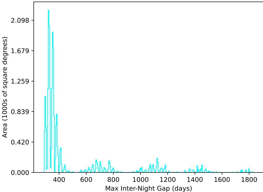
noroll_v3.4_10yrs All sky u band: Max Inter-Night Gap
