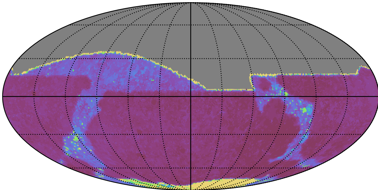
noroll_v3.4_10yrs All sky r band: Max Inter-Night Gap
