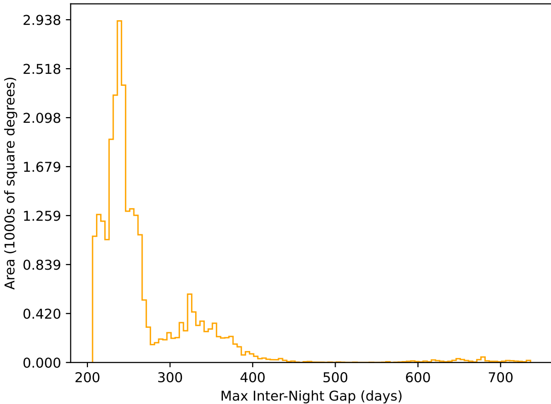
noroll_v3.4_10yrs All sky r band: Max Inter-Night Gap
