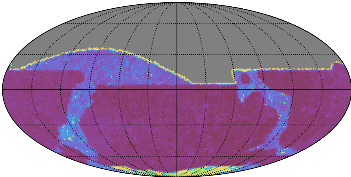
noroll_v3.4_10yrs All sky i band: Max Inter-Night Gap
