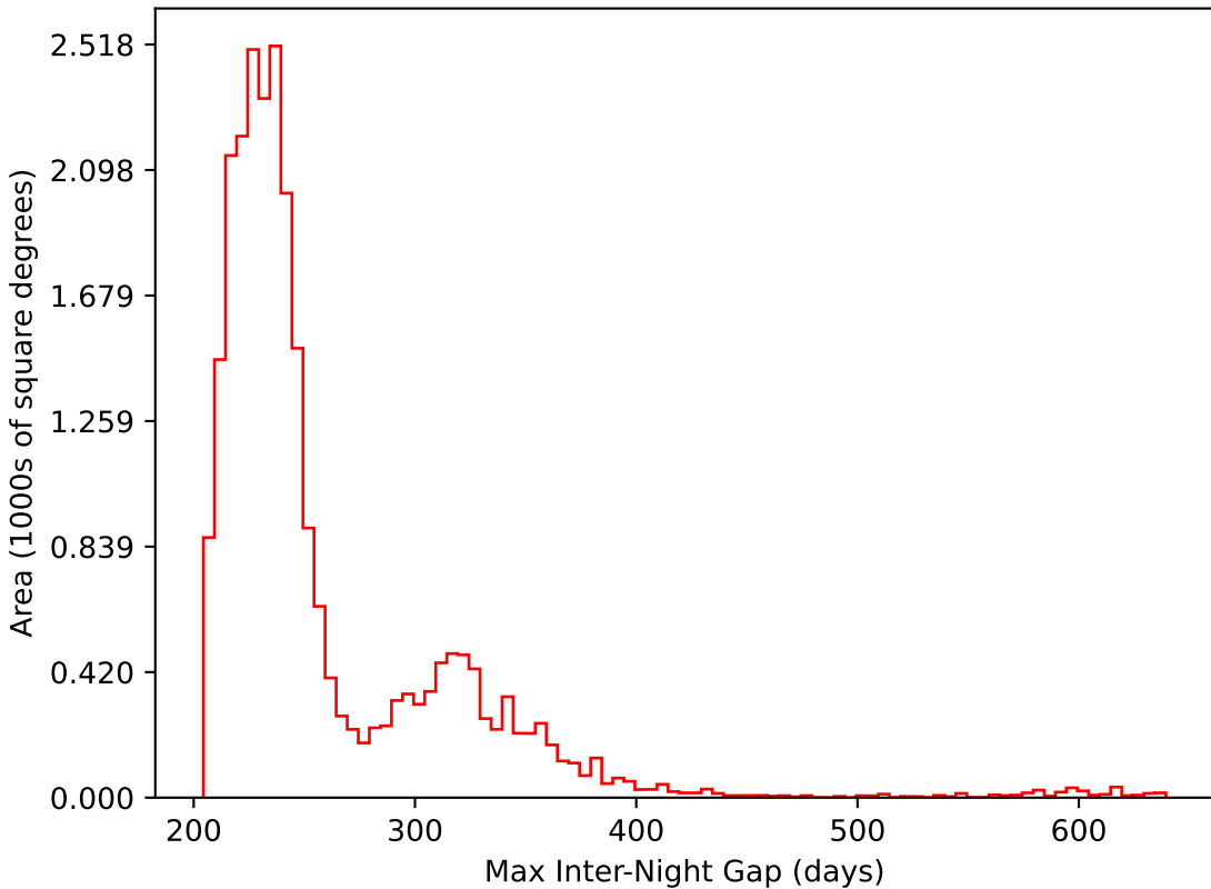
noroll_v3.4_10yrs All sky i band: Max Inter-Night Gap
