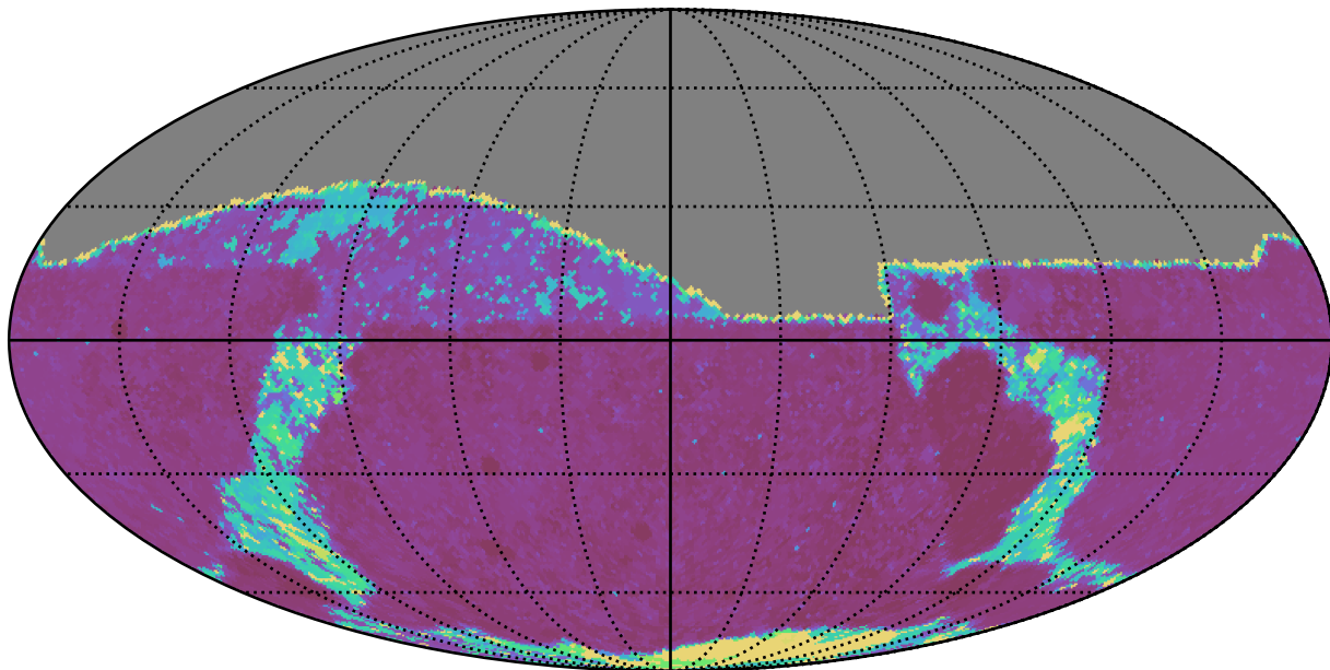
noroll_v3.4_10yrs All sky g band: Max Inter-Night Gap
