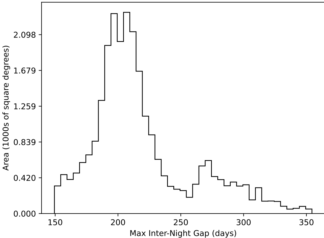
noroll_v3.4_10yrs All sky all bands: Max Inter-Night Gap
