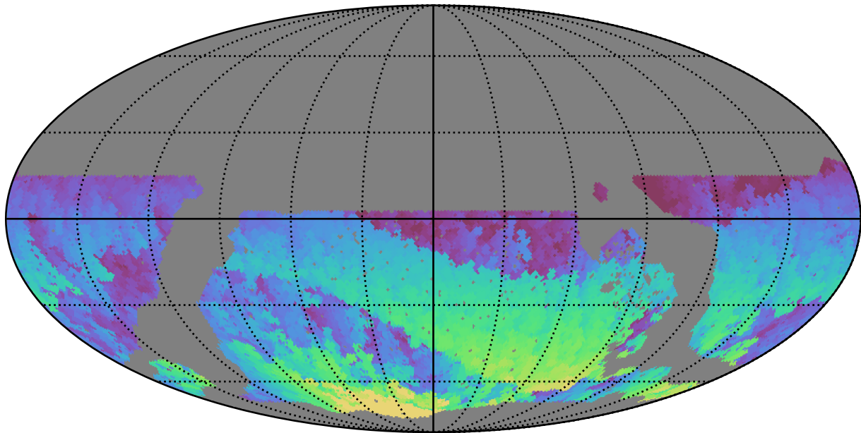
noroll_v3.4_10yrs WFD z band: Max HA
