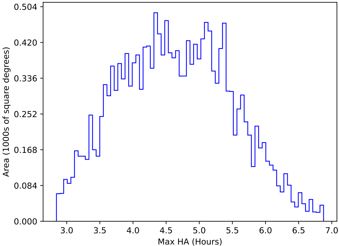
noroll_v3.4_10yrs WFD z band: Max HA
