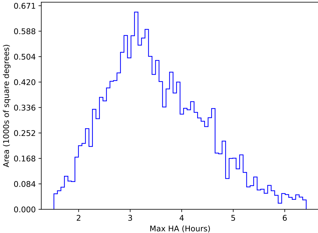
noroll_v3.4_10yrs WFD u band: Max HA
