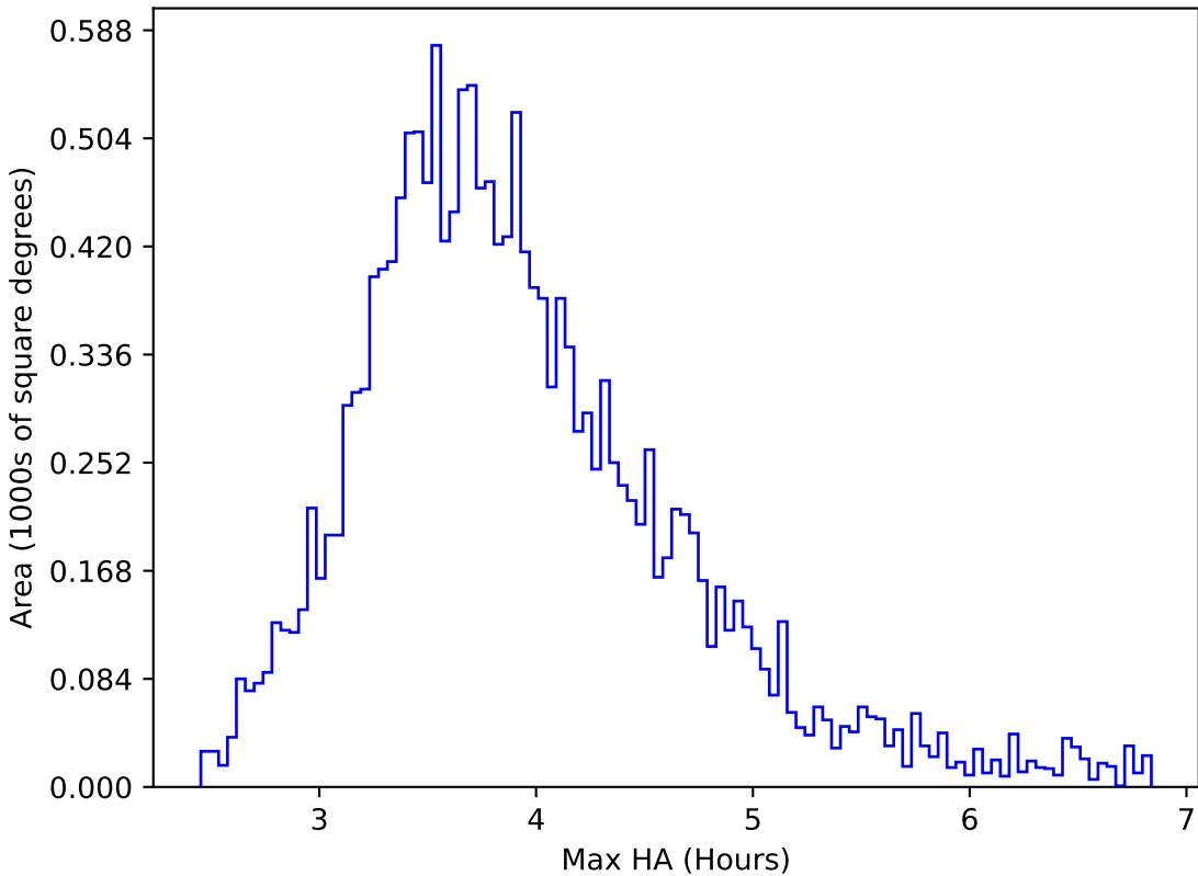
noroll_v3.4_10yrs WFD r band: Max HA
