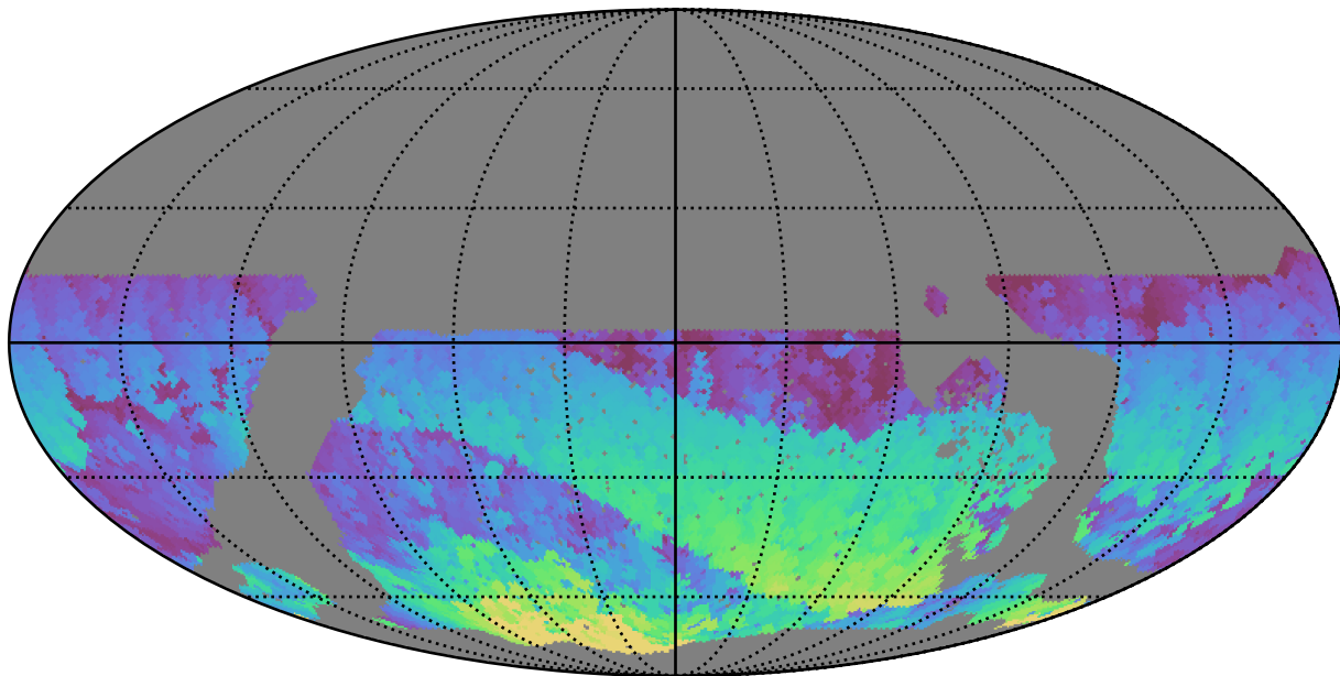
noroll_v3.4_10yrs WFD i band: Max HA
