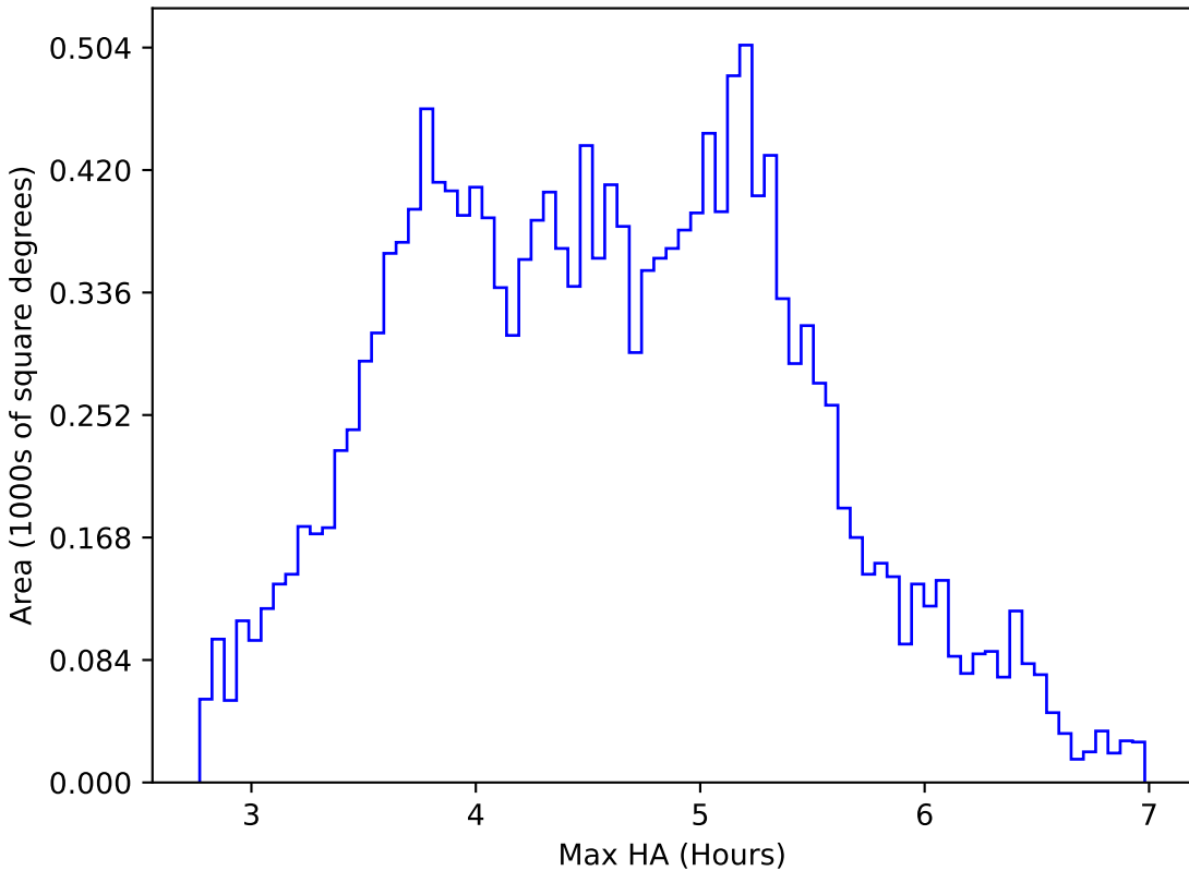
noroll_v3.4_10yrs WFD i band: Max HA
