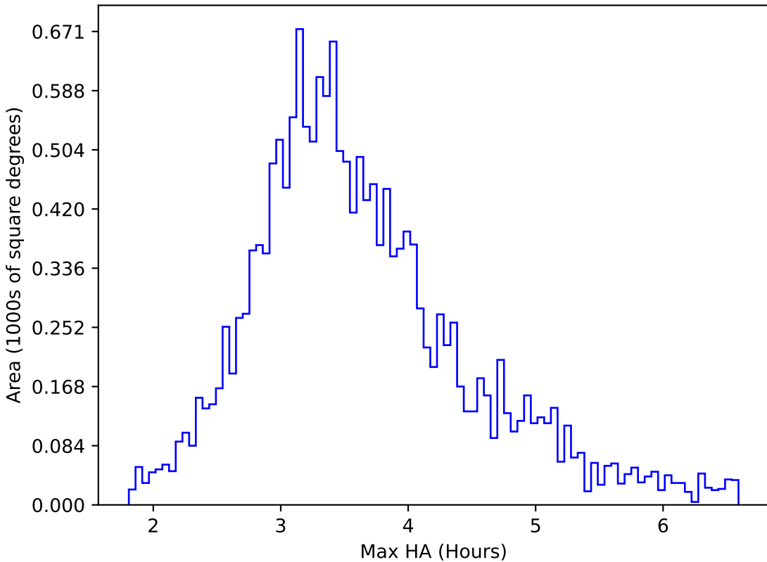
noroll_v3.4_10yrs WFD g band: Max HA
