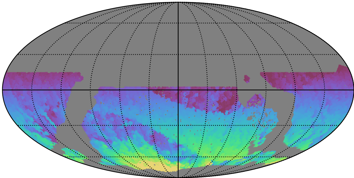
noroll_v3.4_10yrs WFD all bands: Max HA
