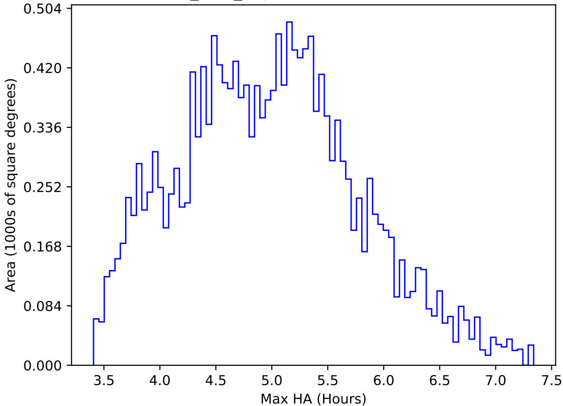
noroll_v3.4_10yrs WFD all bands: Max HA
