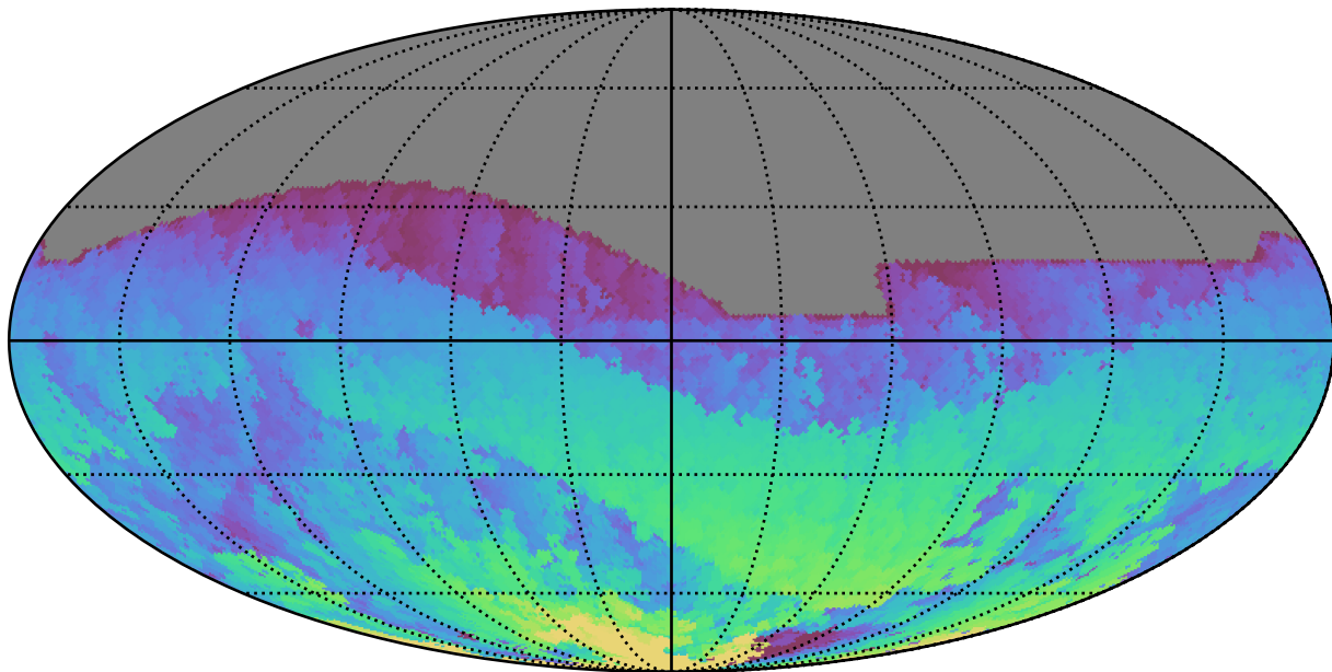
noroll_v3.4_10yrs All sky z band: Max HA
