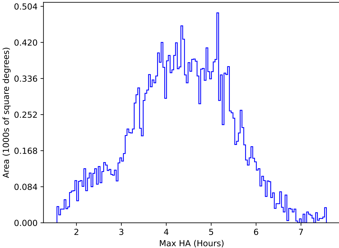
noroll_v3.4_10yrs All sky z band: Max HA
