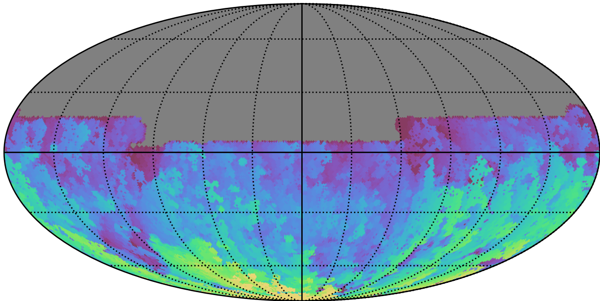
noroll_v3.4_10yrs All sky u band: Max HA
