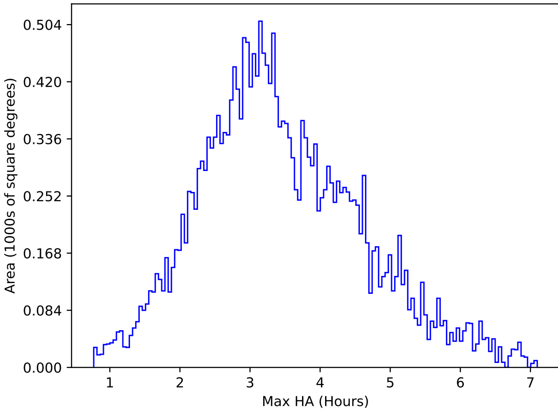
noroll_v3.4_10yrs All sky u band: Max HA
