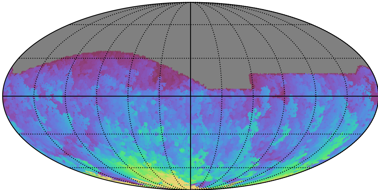
noroll_v3.4_10yrs All sky r band: Max HA
