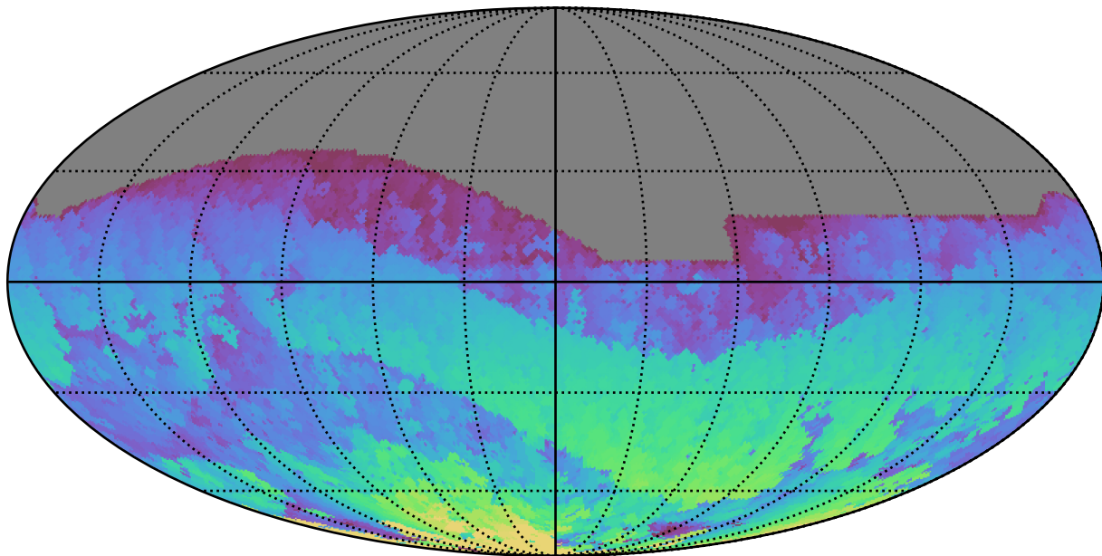
noroll_v3.4_10yrs All sky i band: Max HA
