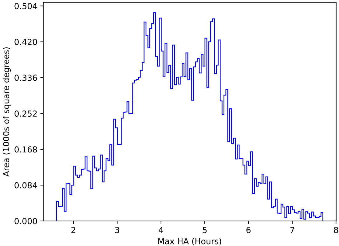
noroll_v3.4_10yrs All sky i band: Max HA
