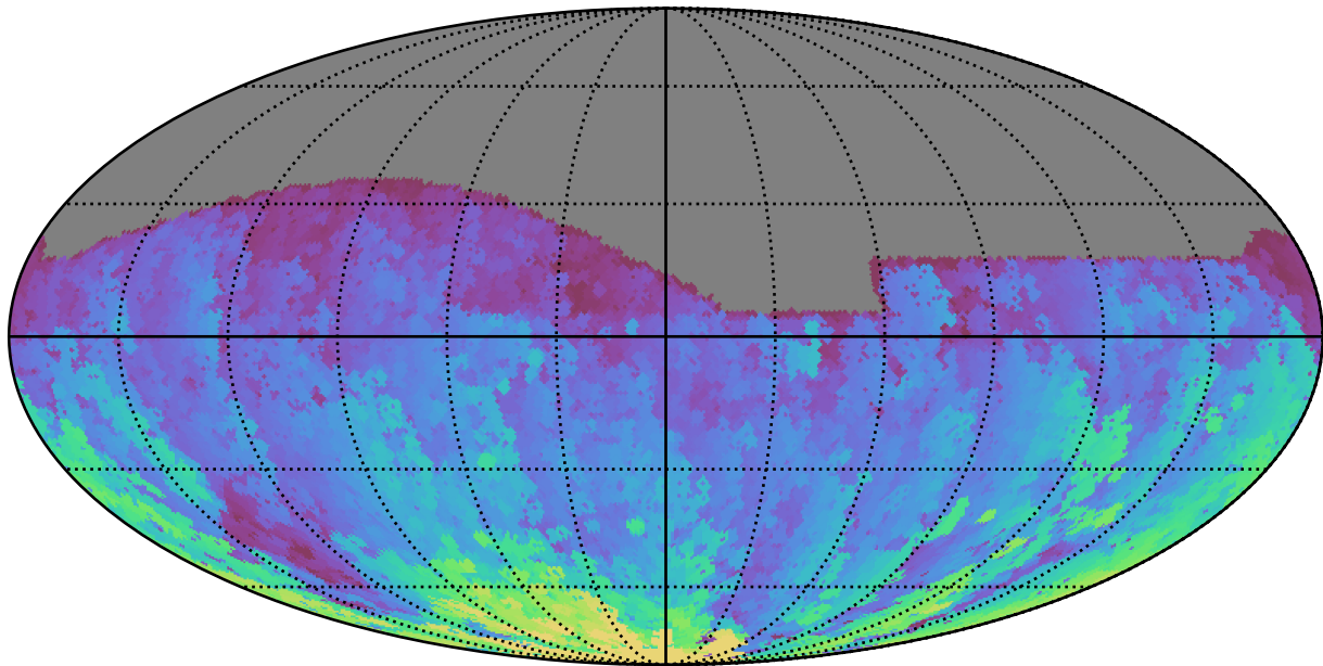
noroll_v3.4_10yrs All sky g band: Max HA
