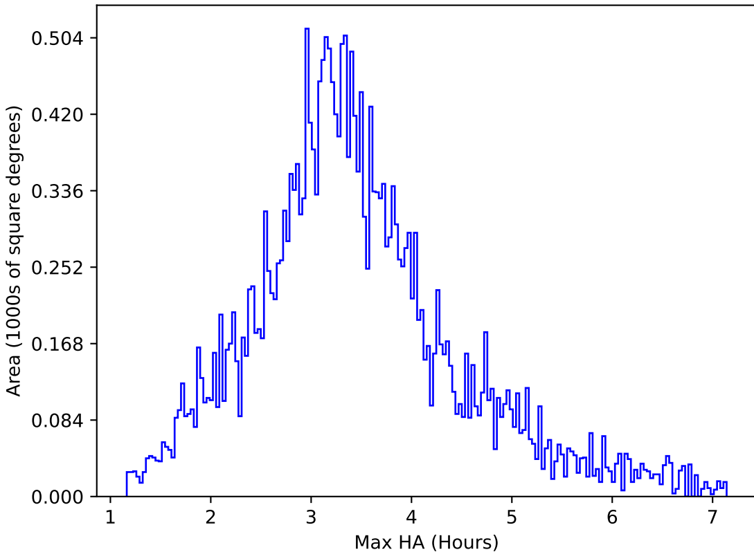
noroll_v3.4_10yrs All sky g band: Max HA
