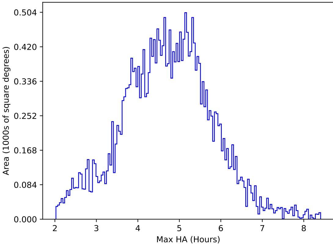
noroll_v3.4_10yrs All sky all bands: Max HA
