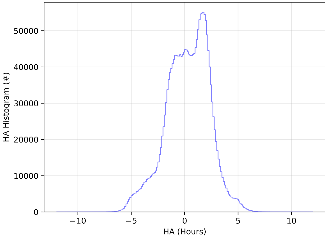
noroll_v3.4_10yrs WFD all bands: HA Histogram
