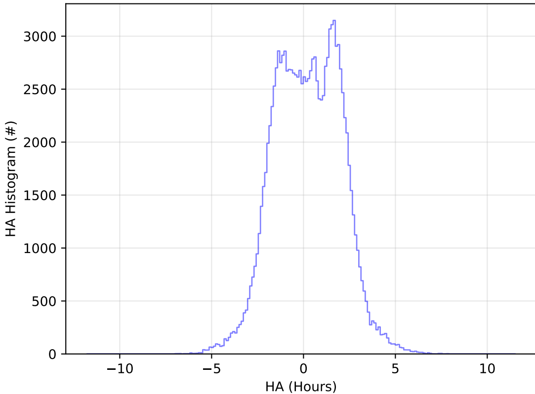
noroll_v3.4_10yrs All sky u band: HA Histogram
