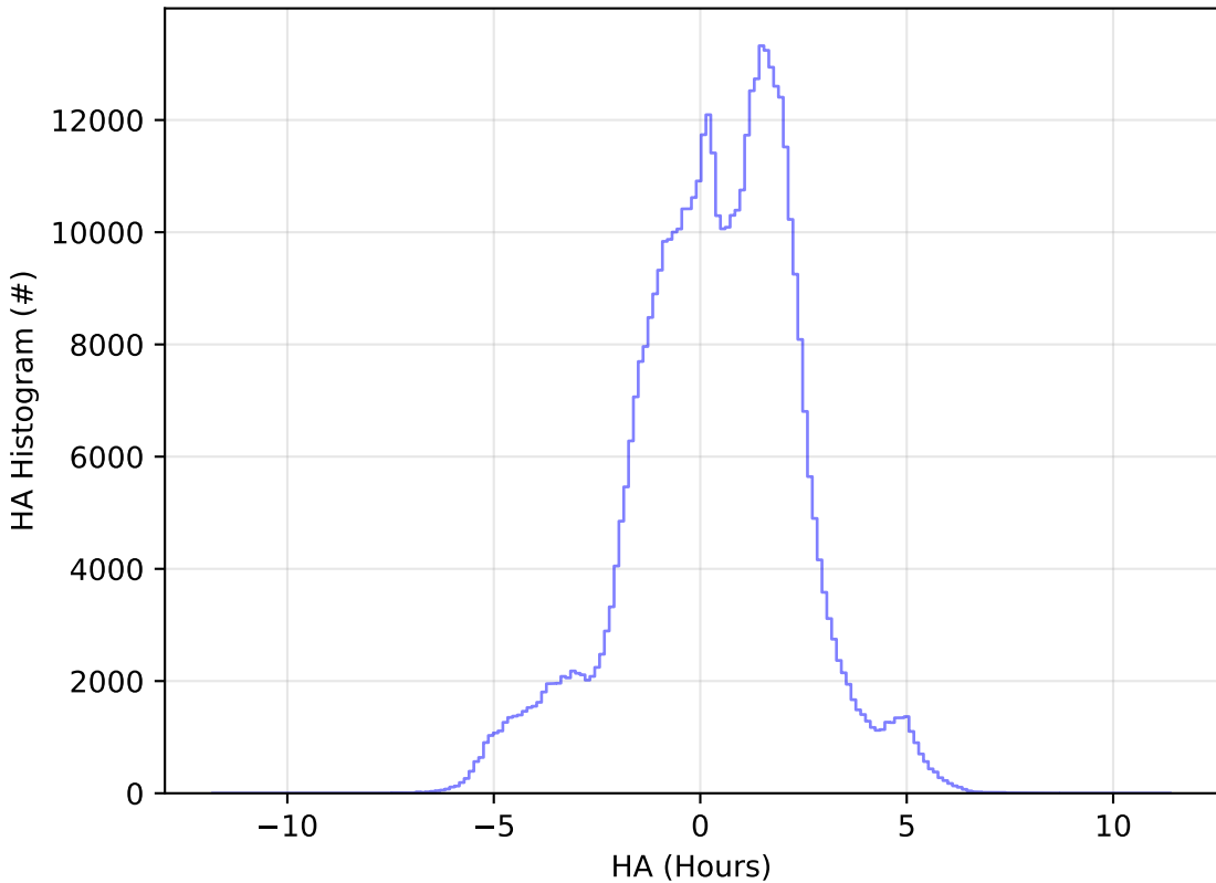
noroll_v3.4_10yrs All sky i band: HA Histogram
