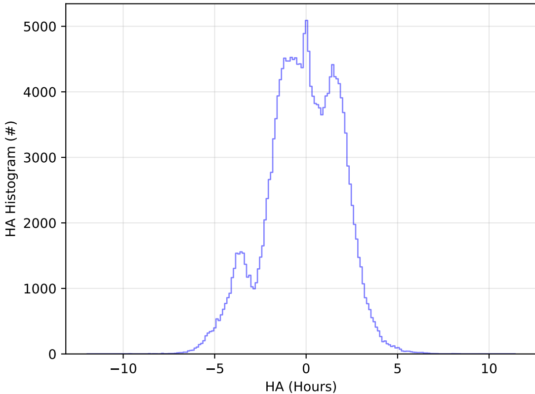
noroll_v3.4_10yrs All sky g band: HA Histogram
