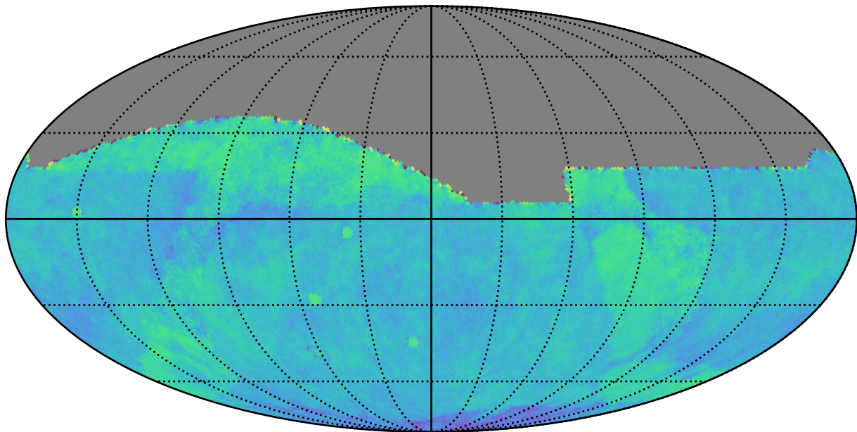
noroll_v3.4_10yrs gri All sky: Fraction of visits in pairs (20-90 min)
