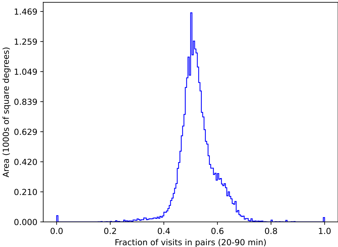
noroll_v3.4_10yrs gri All sky: Fraction of visits in pairs (20-90 min)
